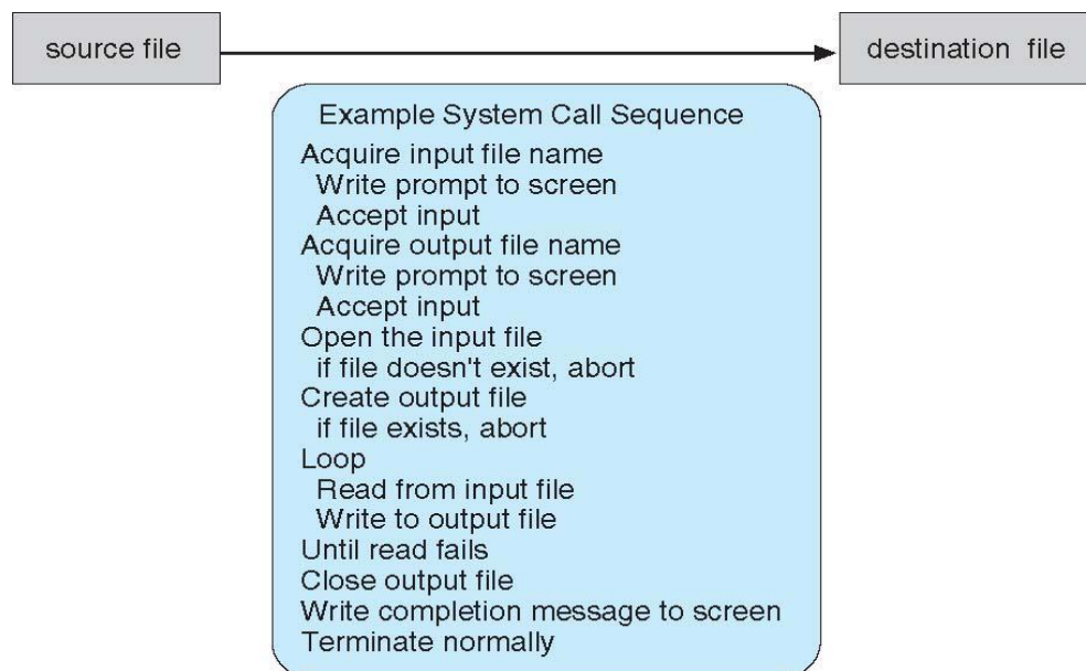
Example of System Calls
