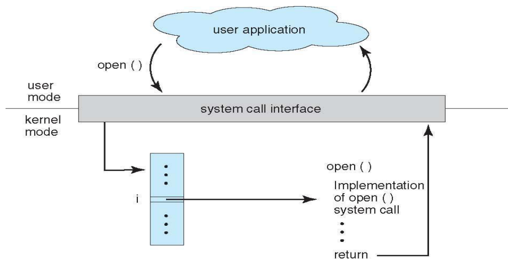
API – System Call – OS Relationship
